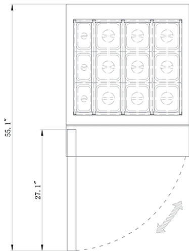
PLAN
