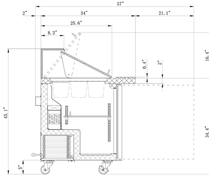
SECTION VIEW
